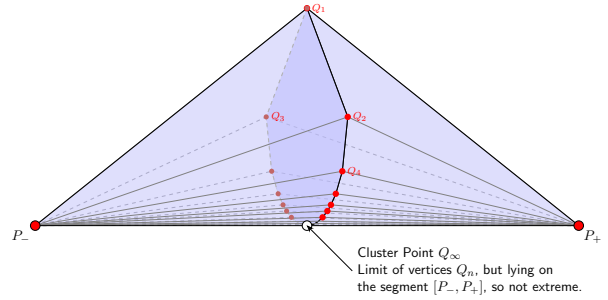
FIGURE 1. Compact convex set C \subseteq \mathbb{R}^3 with non-closed \text{ext}(C)
