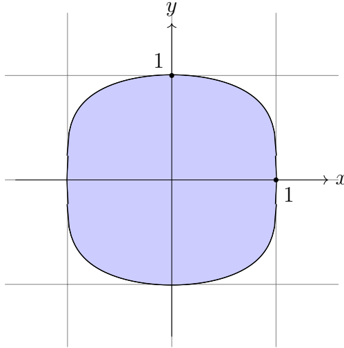
FIGURE 4. Bent TV screen \mathcal{D}_p(1) = \{(x, y) \in \mathbb{R}^2 : 1 - x^2 - y^4 \geq 0\} .
