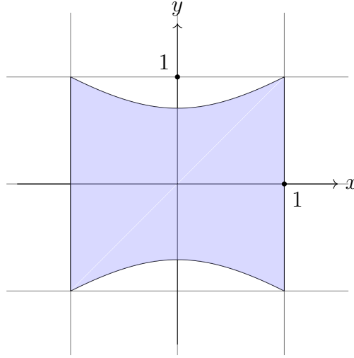
FIGURE 3. The first level component \mathcal{D}_p(1) is clearly not convex in x , hence \mathcal{D}_p is not y^2 -convex.
