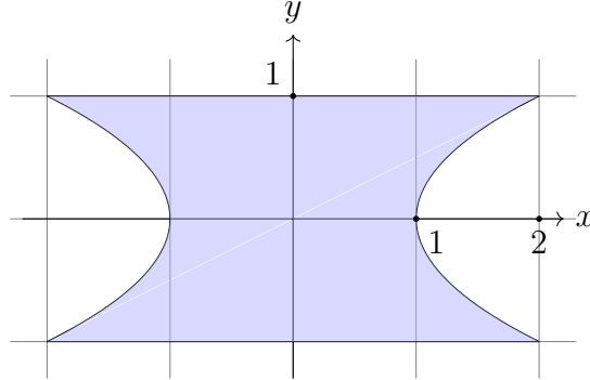
FIGURE 2. The first level component K_1 of \mathbf{K} .
