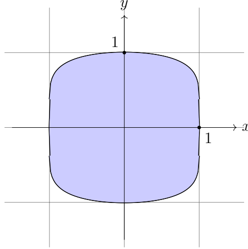
FIGURE 5. Bent TV screen \mathcal{D}_p(1) = \{(x, y) \in \mathbb{R}^2 : 1 - x^2 - y^6 \geq 0\} .
